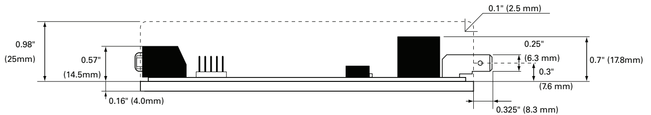
FIGURE 14. LDC22xx side view and dimensions
