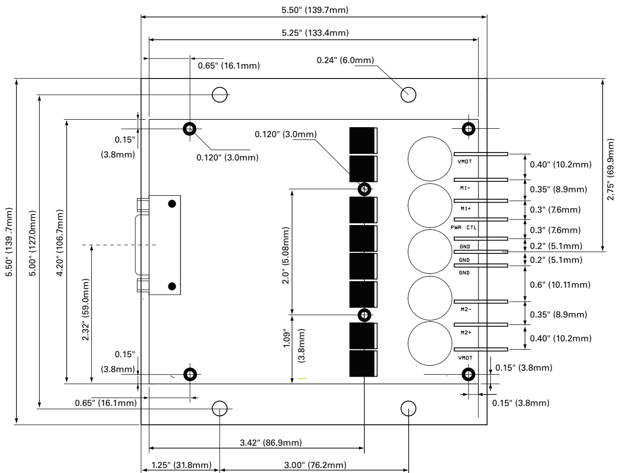
FIGURE 15. LDC22xx top view and dimensions
