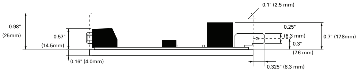
FIGURE 17. LBL13xx side view and dimensions
